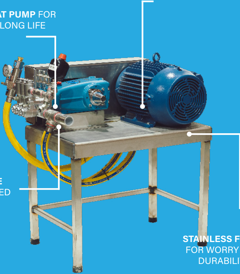
ELECTRIC MOTOR FOR EXHAUST FREE OPERATION
