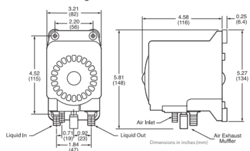
Dimensional Drawing
